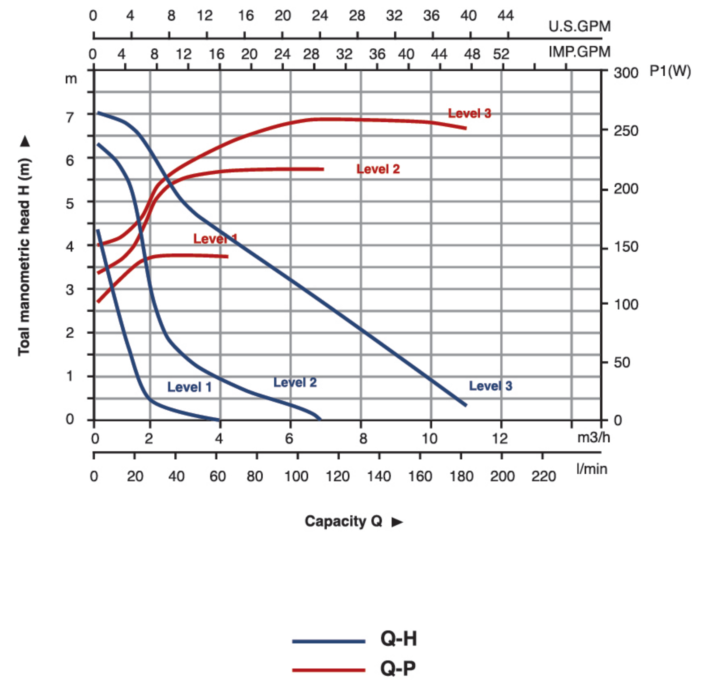
ACP 40-80F/250
