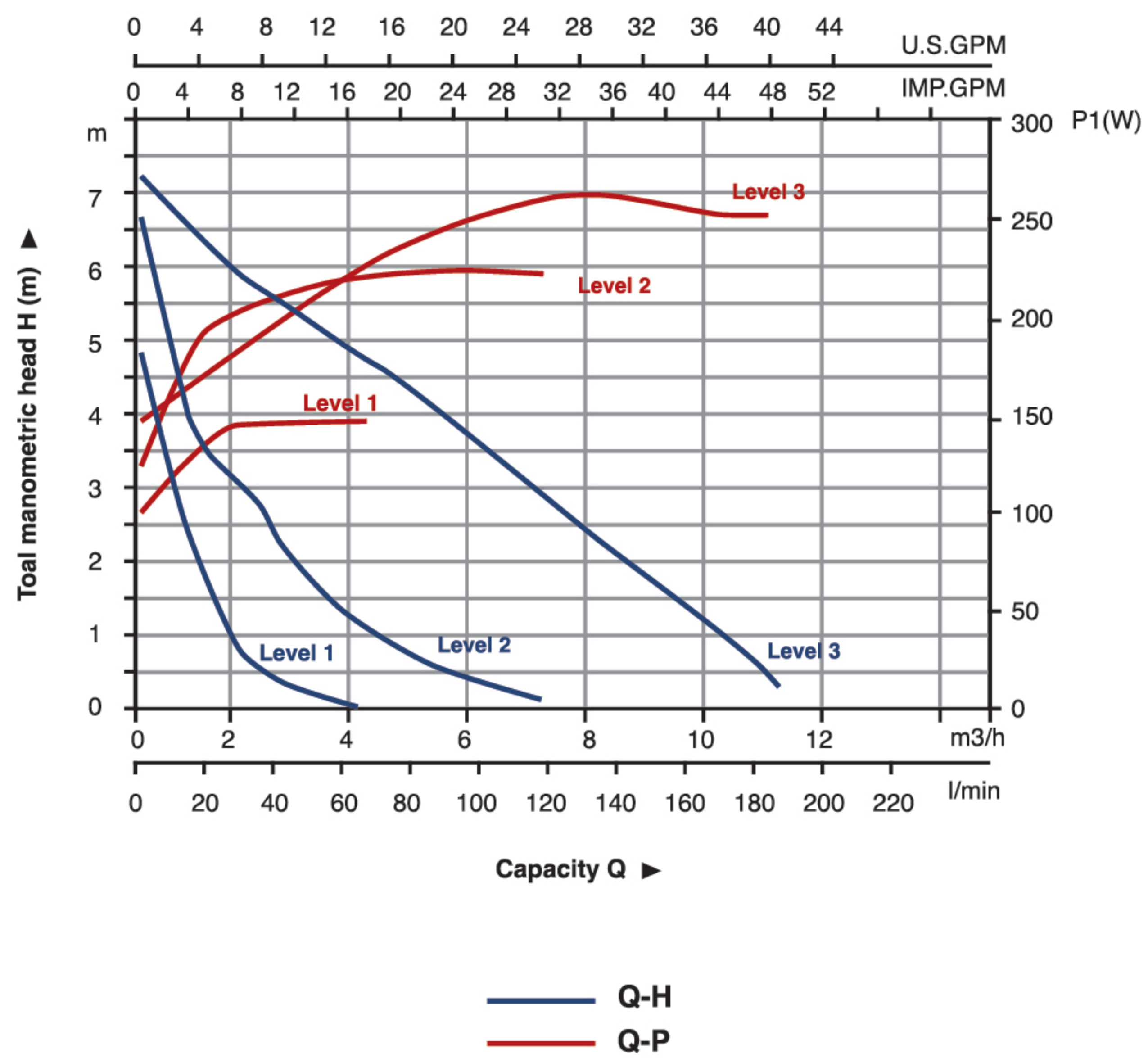
ACP 36-80F/200
