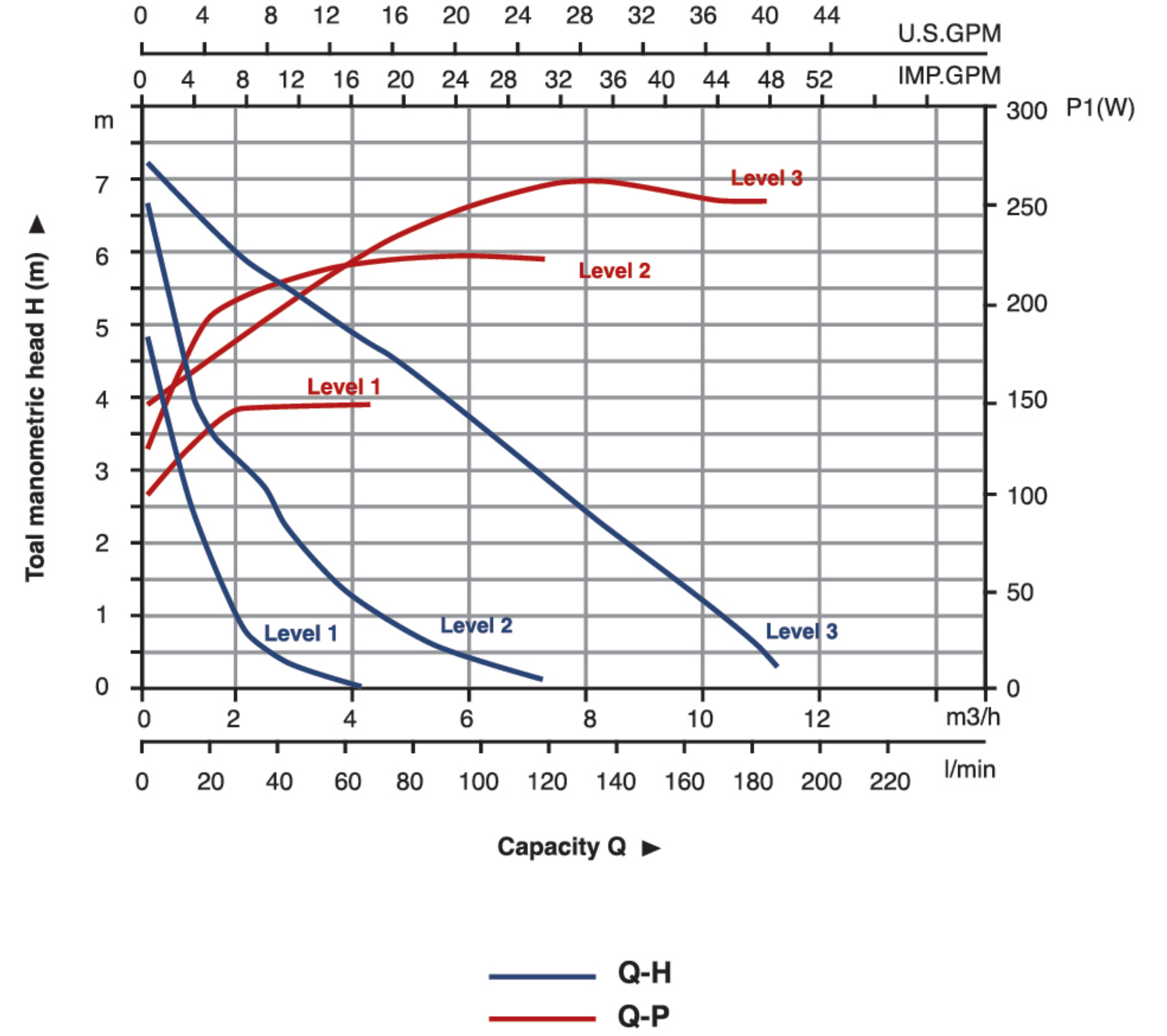
ACP 32-80/180
