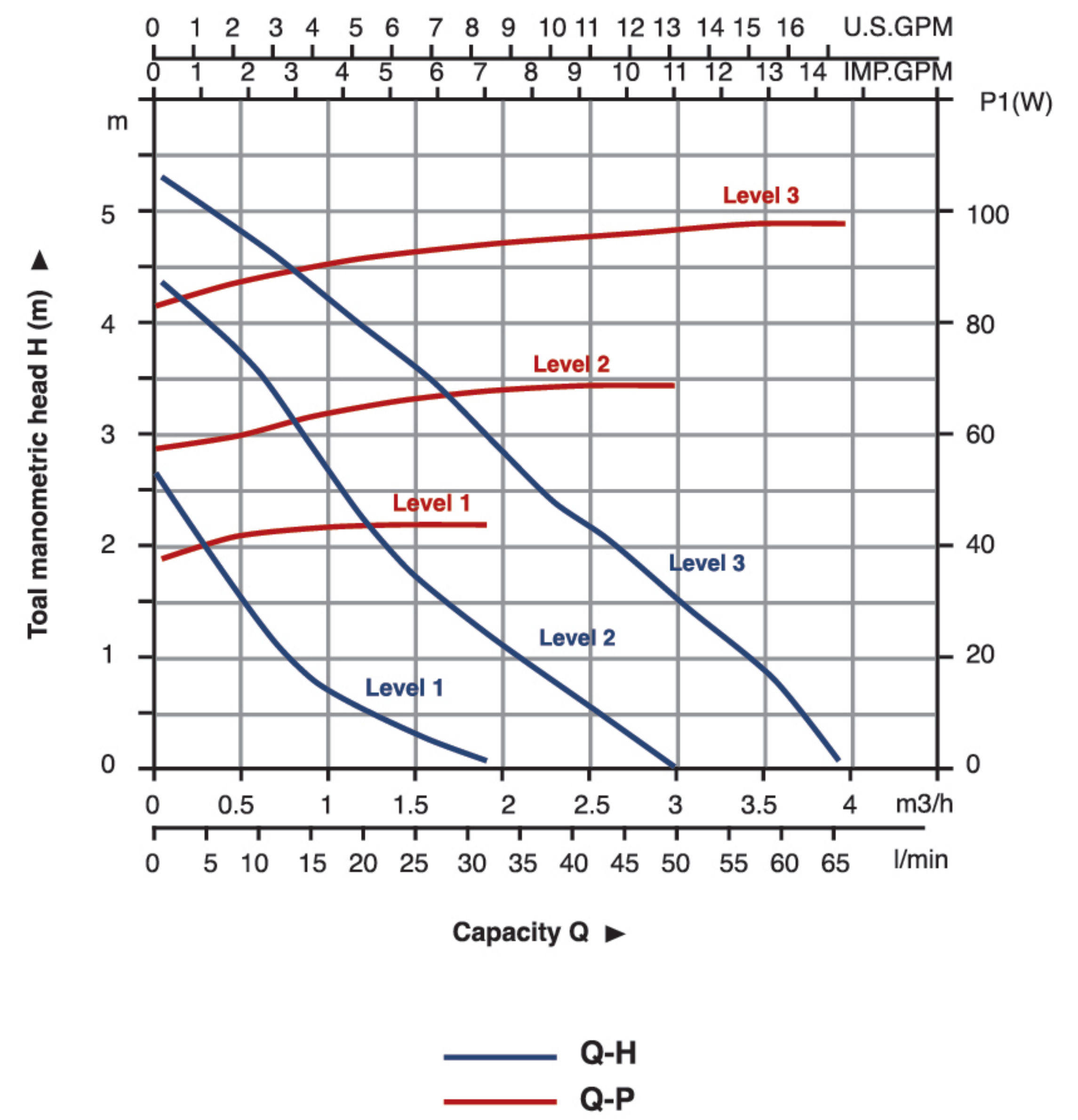
ACP 25-60/180
