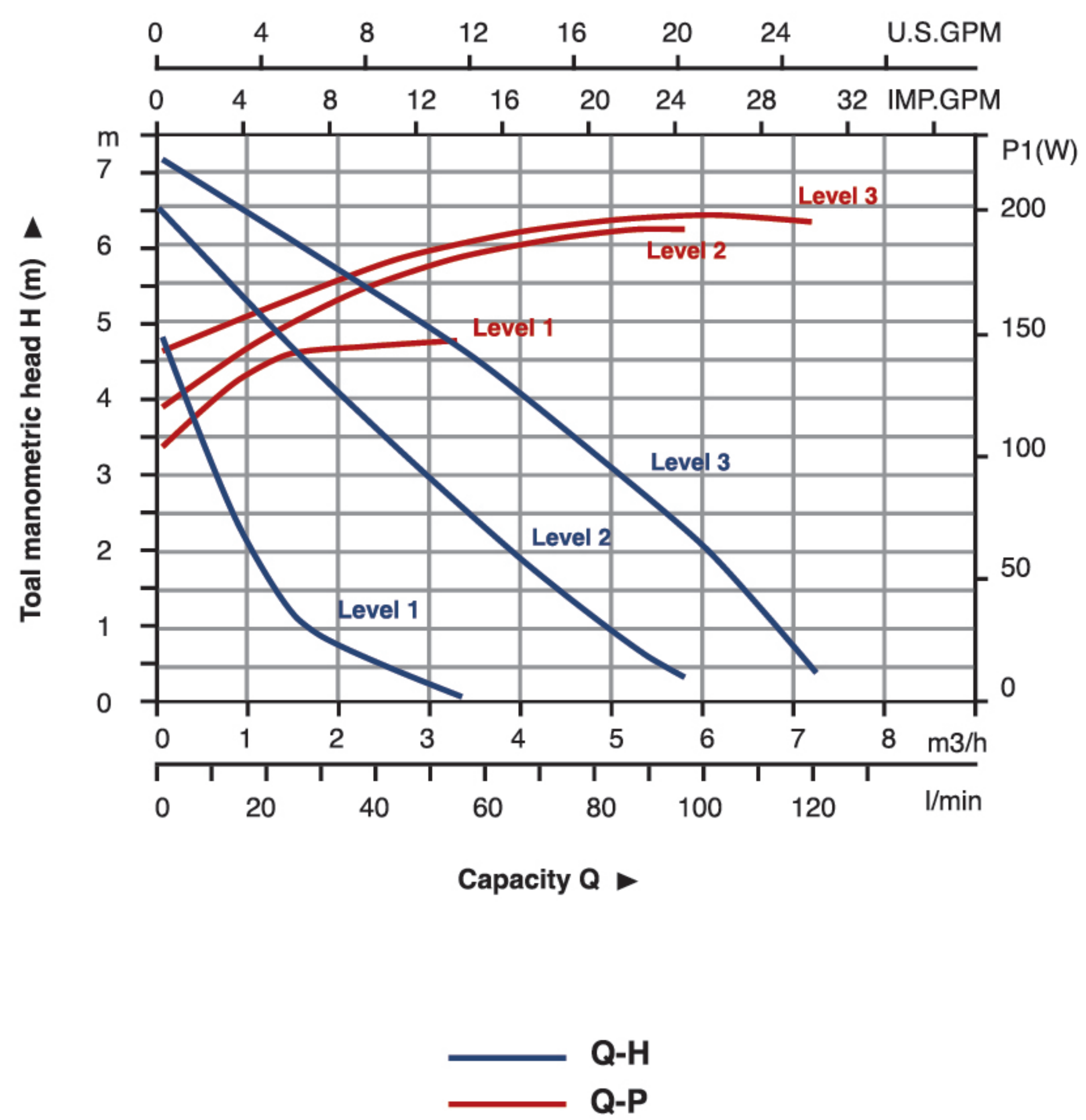
ACP 25-80/180
