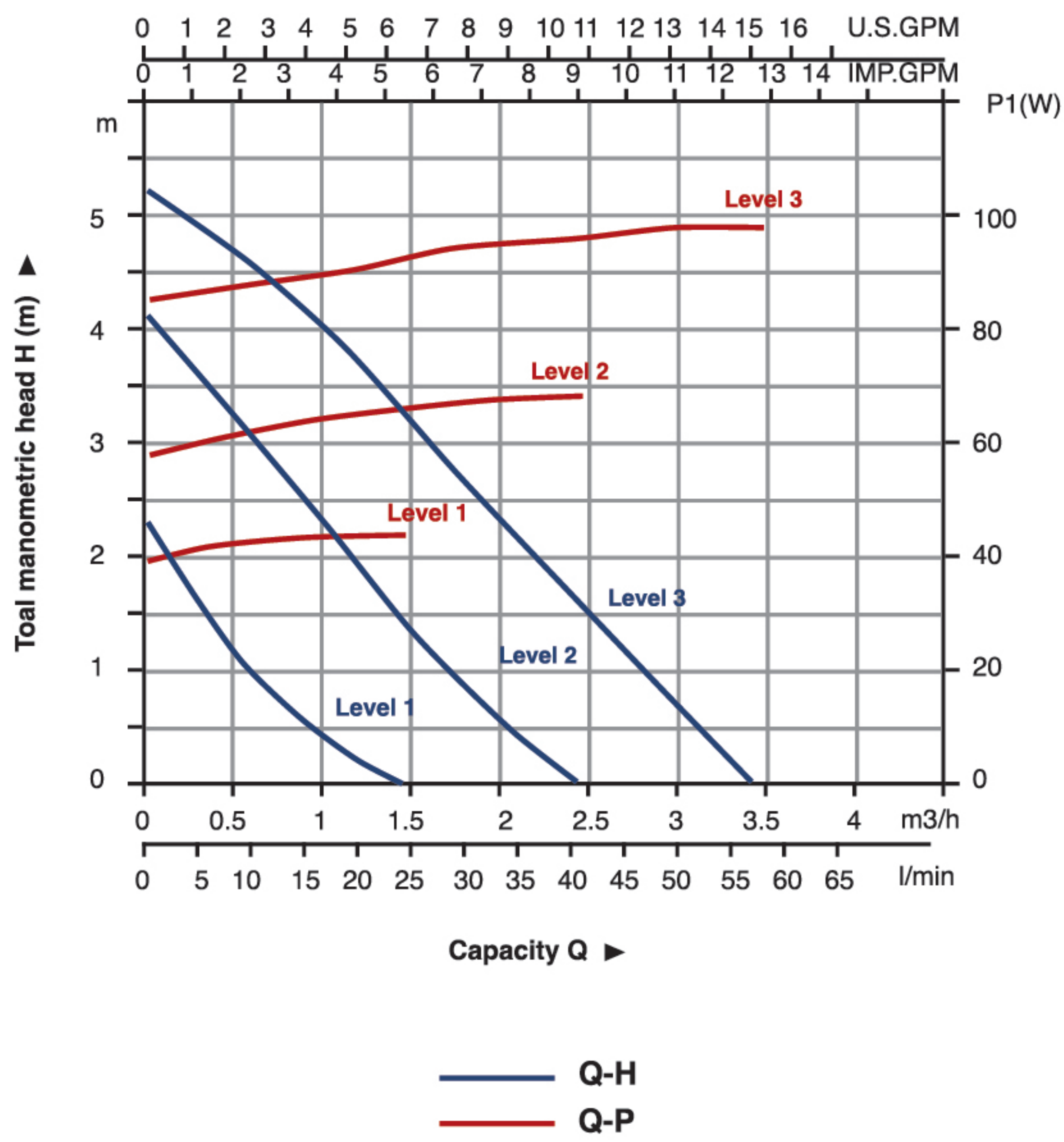
ACP 25-60/130
