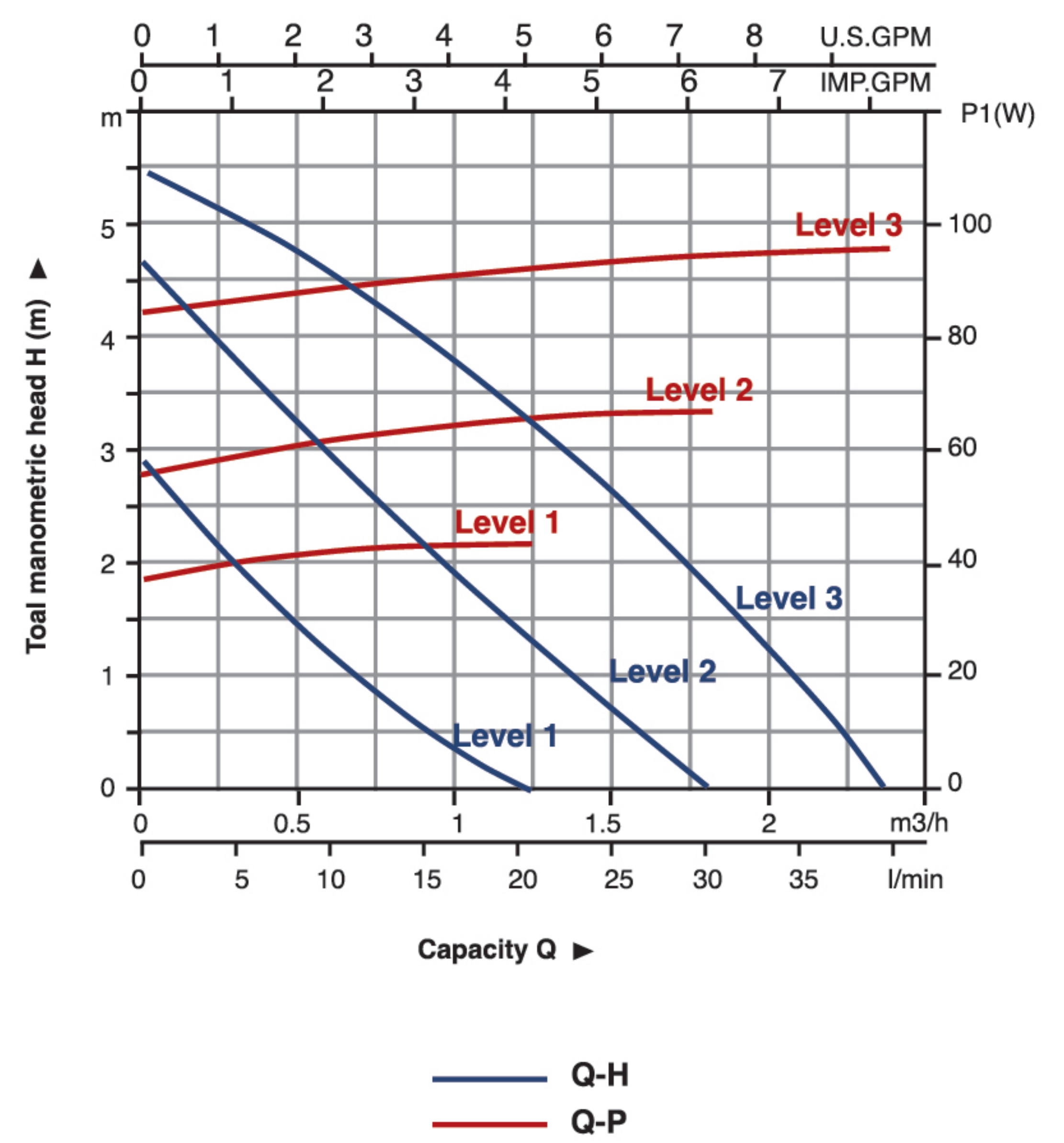
ACP 15-60/130
