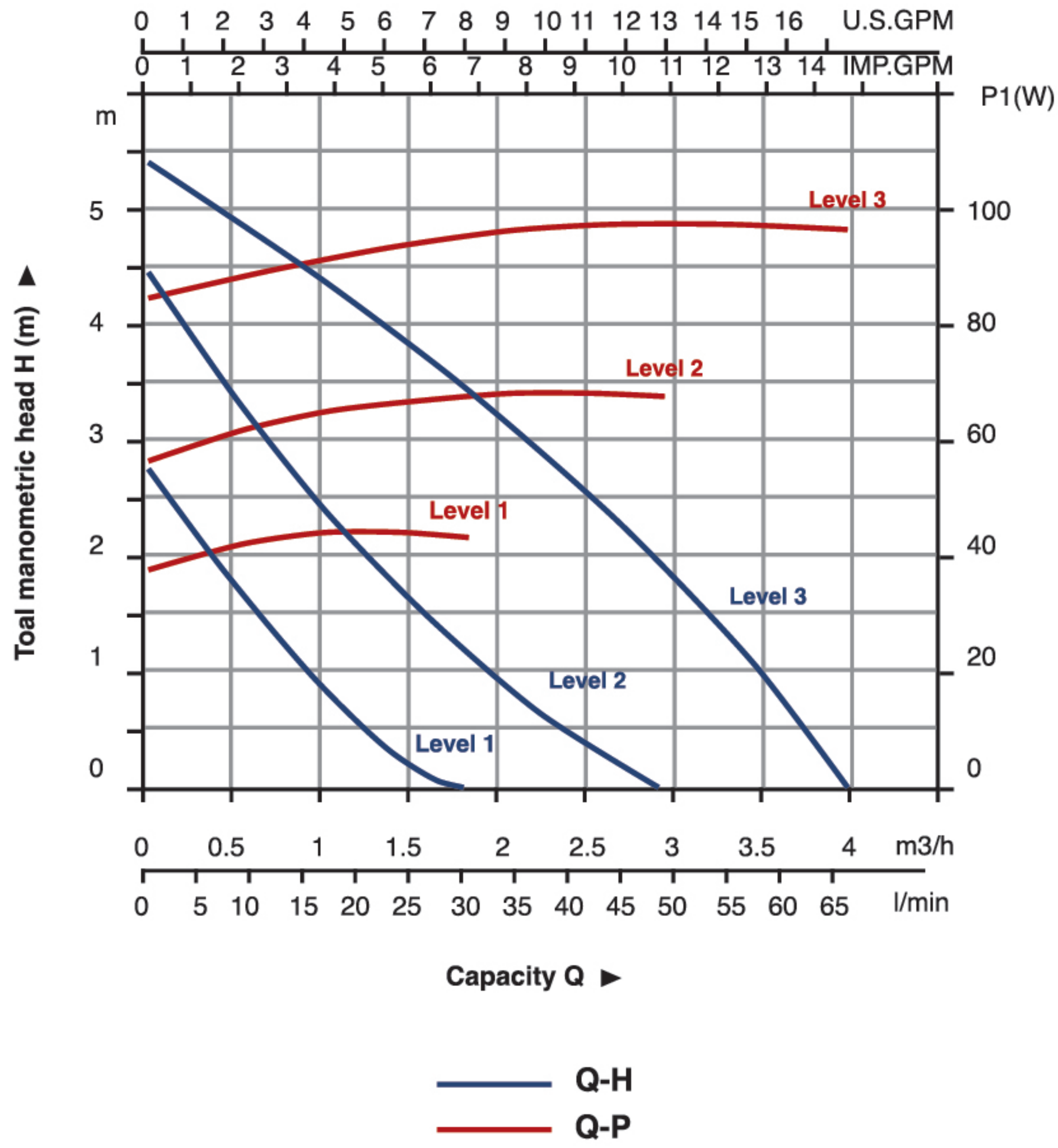
ACP 32-60/180
