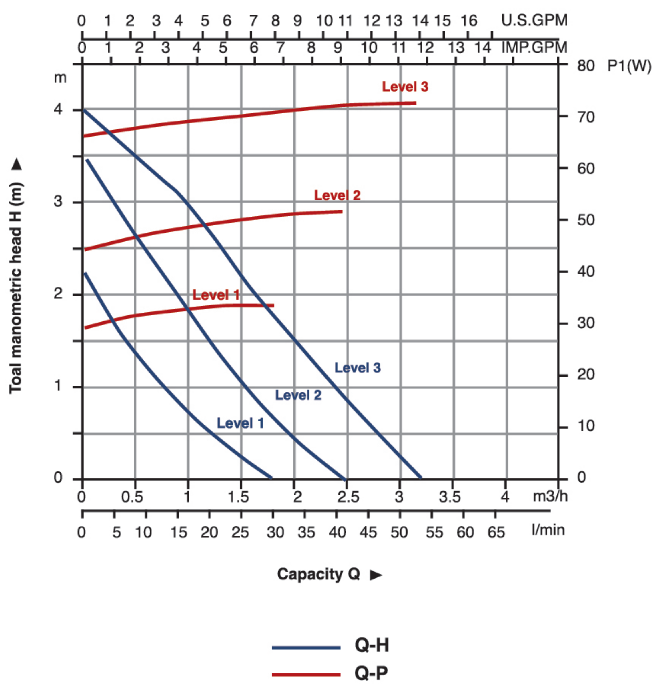
ACP 25-40/130
